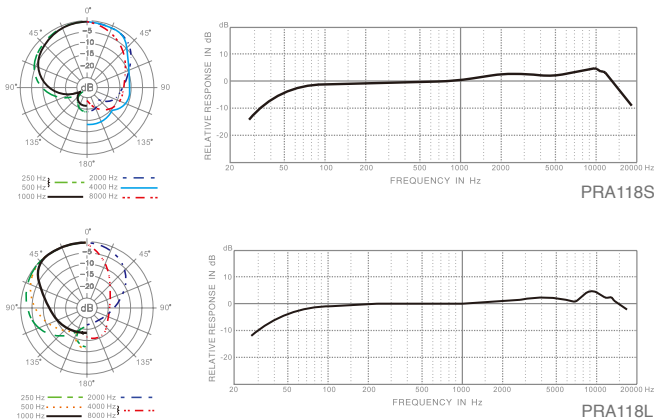
PRA118 Frequency Response ( Shotgun )
