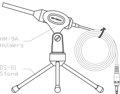
Dimensions (Figure 3)
